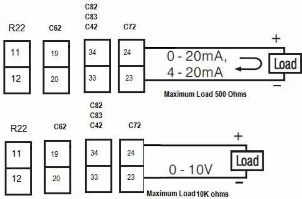
2- 43 Retransmission Wiring
