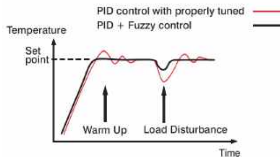
1- 1 Fuzzy PID Control
